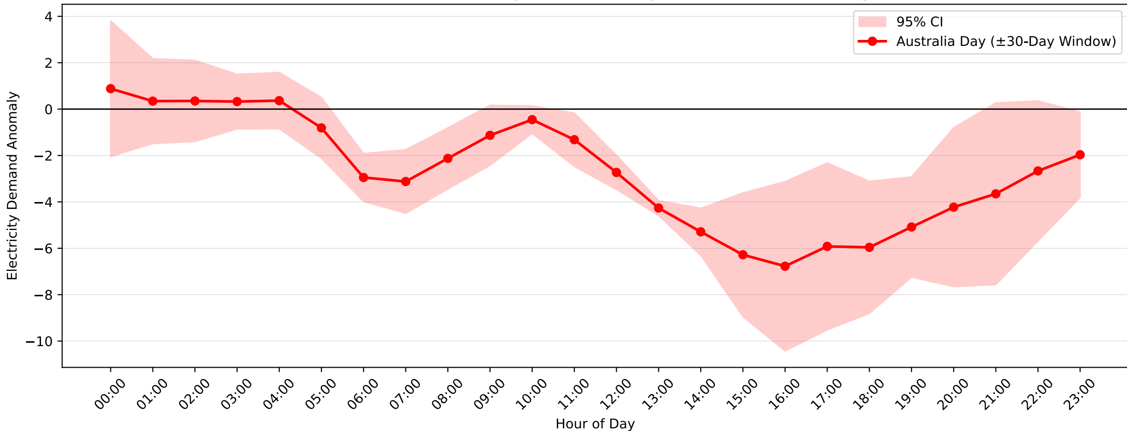
Pennant Hills Demand Anomaly: Australia Day (2015-2016, \pm 30 -Day Window)
