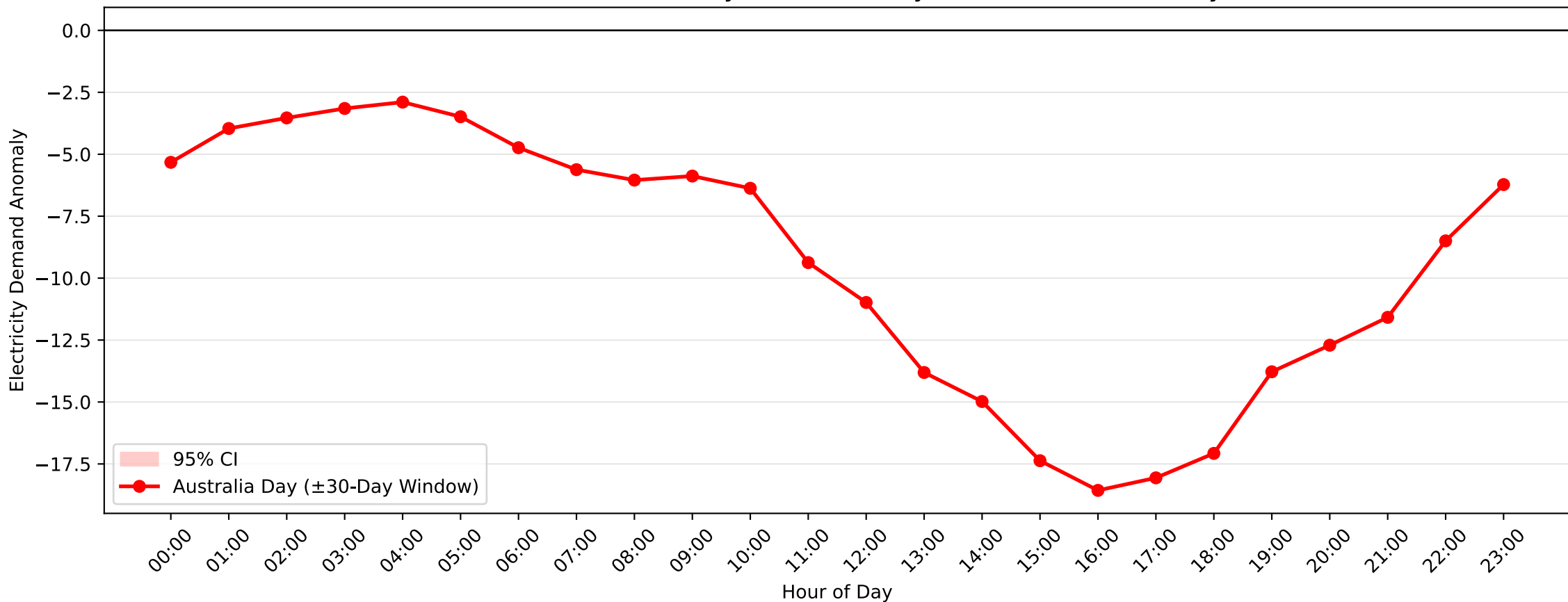
Pennant Hills Demand Anomaly: Australia Day (2017-2018, \pm 30 -Day Window)
